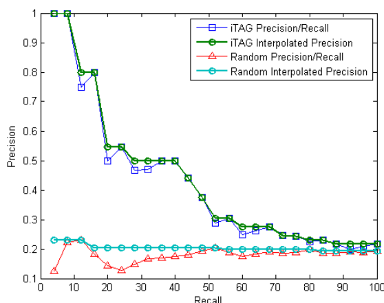
Figure 10 compares the iTAG vs. random approaches for McCain's speeches in terms of precision and recall.
