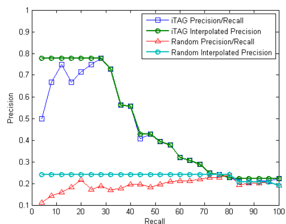
Figure 9 compares the iTAG vs. random approaches for Obama's speeches in terms of precision and recall.
