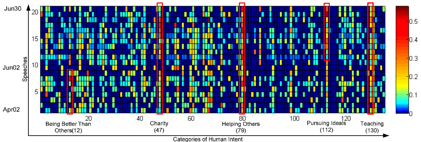
Figure 4 provides an overview of intent annotations for 21 speeches given by Barack Obama in April and June 2008. Selected categories which are predominant over a certain period of time are highlighted.
