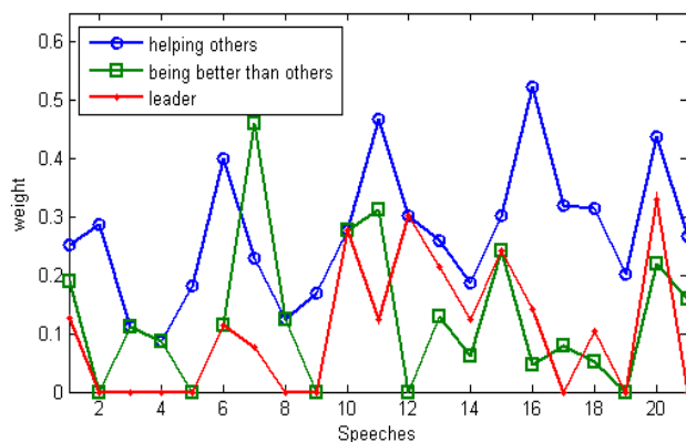
Figure 7 illustrates temporal evolution chart of three selected Intent Annotations “Helping Others”, “Being Better Than Others” and “Leader” over 21 speeches given by B. Obama.
