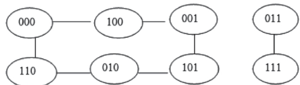
Figure 4. Conflict graph
